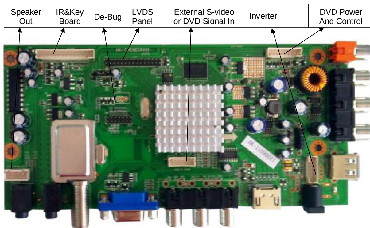
Below Picture is for Front View of HK-T.RENEC8V01
