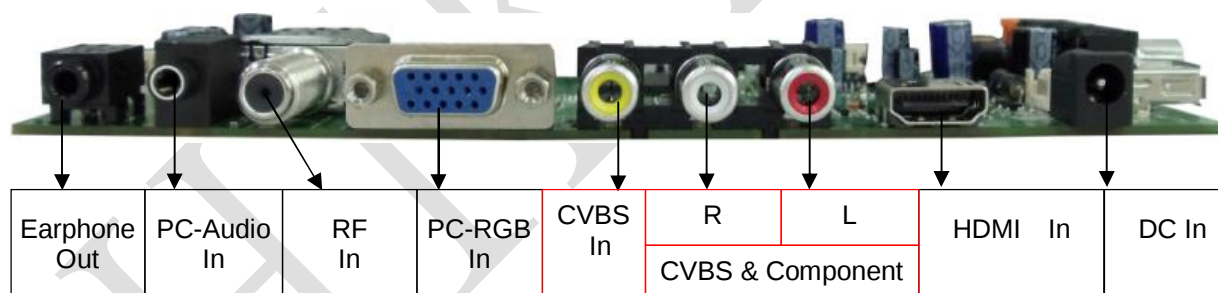
Below Picture is for Side View of HK-T.RENEC8V01
