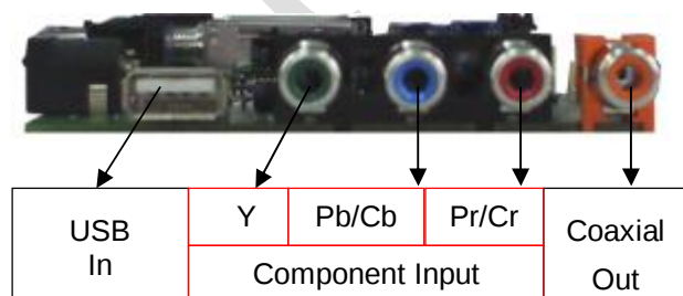
Below Picture is for Side View of HK-T.RENEC8V01
